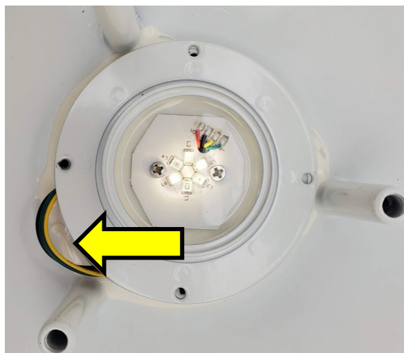
Be sure there is NO wires between the cover and seal or there will be a gap to let water in.
