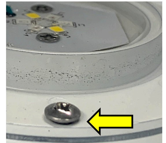
After tightening all 3 screws: GO BACK and verify if any additional tightening is needed
